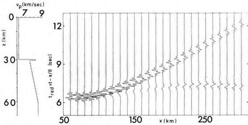
Fig. 13. The same model as in Figure 12, but with Q_p = \infty and a thin high-velocity layer on top of the gradient zone ( h = 625 m, r_p = 8.2 km/s). The low-frequency tunnel wave is now on the prograde branch of refracted P . High frequencies start to arrive on this branch beyond 200 km
