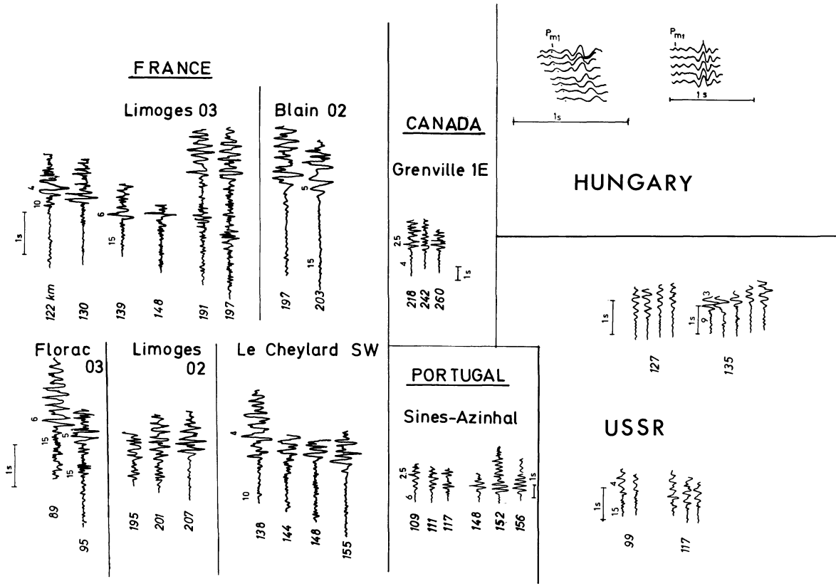
Fig. 10a. Examples of low-frequency P_mP phases following high frequency precursors from various continental parts of the world. Dominant frequencies are indicated at the phases and distances at the beginning of every phase. Seismogram samples are from France (Sapin and Prodehl, 1973); Canada (Berry and Fuchs, 1973); Portugal (Mueller et al., 1973); Hungary (Mituch and Posgay, 1972); U.S.S.R. (Zverev and Tulina, 1971)
