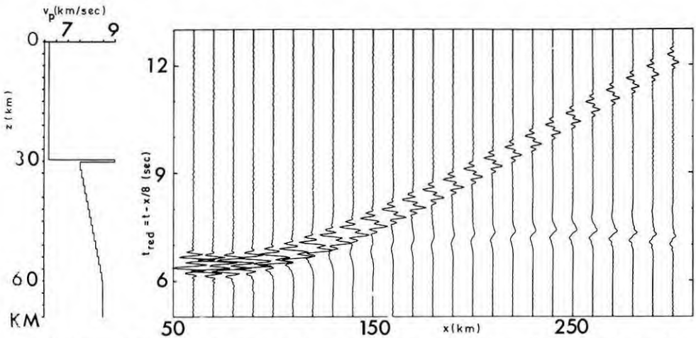
Fig. 14. The same model as in Figure 13, but with r_p = 9.0 km/s in the thin layer. High frequencies on the refracted P -branch are strongly suppressed. The wave field is very similar to that in Figure 12
