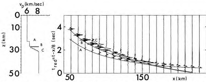
Fig. 9. Synthetic seismogram section for a model of the crust-mantle transition which simulates the observed frequency behaviour
