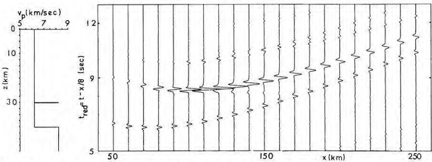
Fig. 5. Thickness of the thin layer h = 100 m, otherwise as Figure 3
