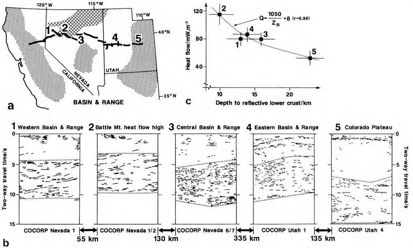
Fig. 2. a Map of western USA to show COCORP lines in relation to heat flow provinces. Cross-hatching : heat flow \geq 105 \text{ mW} \cdot \text{m}^{-2} ; dots : heat flow \leq 63 \text{ mW} \cdot \text{m}^{-2} ; blank area : intermediate heat flow values (Lachenbruch and Sass, 1977). Numbers 1–5 show locations of data segments illustrated in Fig. 2b. b Data segments along the COCORP Basin and Range survey. The reflective lower crust has been shown to be essentially continuous between the data segments illustrated. Each data segment is 25 km long, and is located by its number in Fig. 2a. Data redrawn from Hauge et al. (1987), Potter et al. (1987b), Allmendinger et al. (1983) and Mayer and Brown (1986). Dotted lines mark the interpreted top of the reflective lower crust and the interpreted reflection Moho. c Plot of heat flow vs. depth to the top of the reflective lower crust. Values plotted (see Table 1) are derived from the full dataset located in Fig. 2a rather than the 25-km data segments illustrated in Fig. 2b
