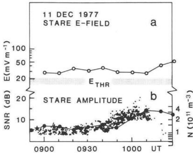
Fig. 1 a and b . Data for the event 11 Dec 1977: a STARE E field magnitude, b STARE backscatter amplitude from the Finnish radar (scattered small dots), as well as the electron density from the MMK ionosonde (heavy dots) and from the TRO ionosonde (star)
