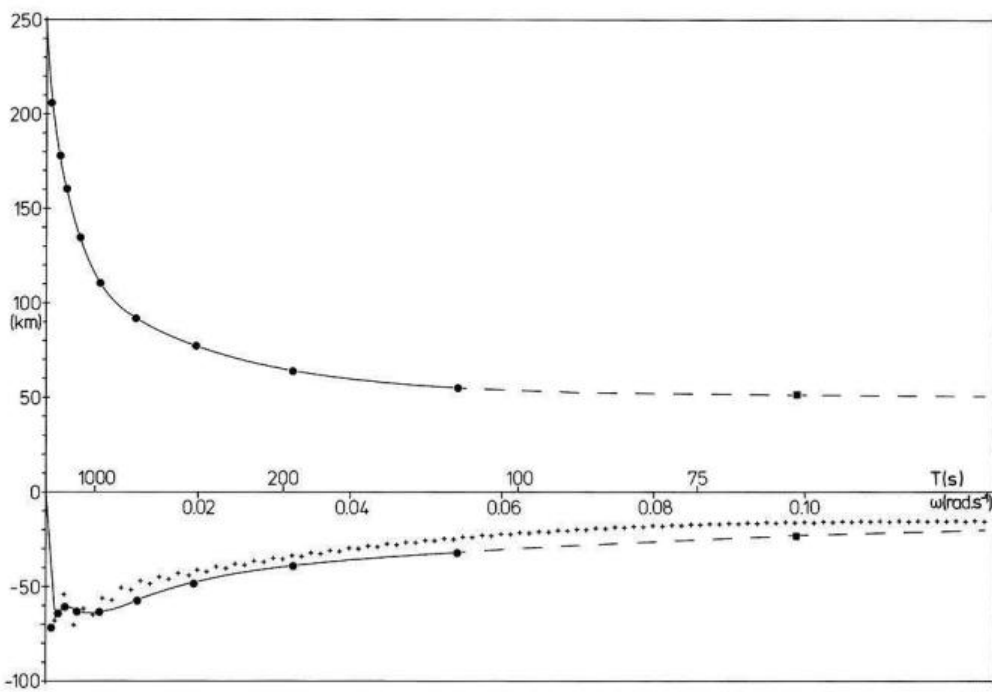
Fig. 8. Interpolation of g (positive) and -h (negative) in the observation range given by solid lines. Dashed lines are the extrapolations of these functions to higher frequencies using the parameters from a two-layer model as aids (squares). Crosses are the function g_H = -\mathcal{H}\{g\} , the Hilbert transform of g
