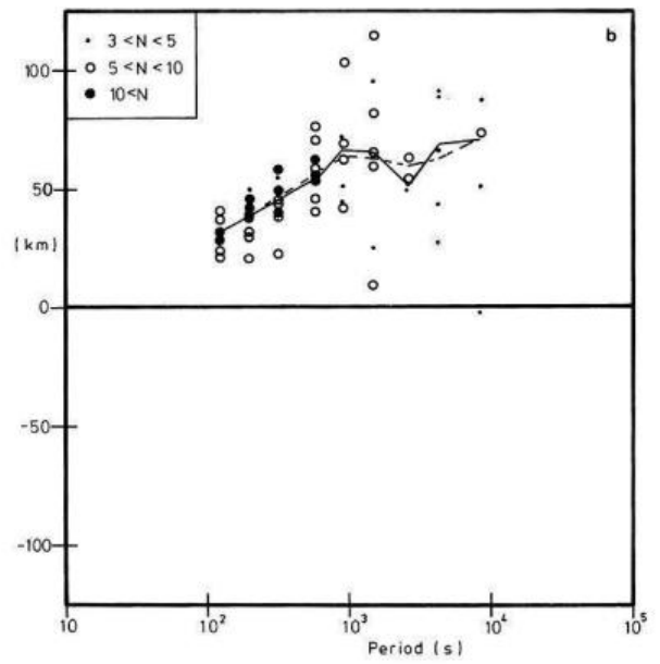
Fig. 7. a Individual event determinations of g with the corresponding value of the normalised transformed ordinary coherence being indicated by symbol type: \bullet \equiv 3 < N < 5 ; \circ \equiv 5 < N < 10 ; \bullet \equiv 10 < N . The full line indicates the weighted ensemble average, and the dashed line is the Hanning-smoothed average. b As (a) but for h
