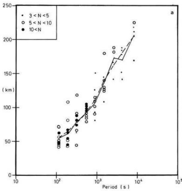
Fig. 7. a Individual event determinations of g with the corresponding value of the normalised transformed ordinary coherence being indicated by symbol type: \bullet \equiv 3 < N < 5 ; \circ \equiv 5 < N < 10 ; \bullet \equiv 10 < N . The full line indicates the weighted ensemble average, and the dashed line is the Hanning-smoothed average. b As (a) but for h
