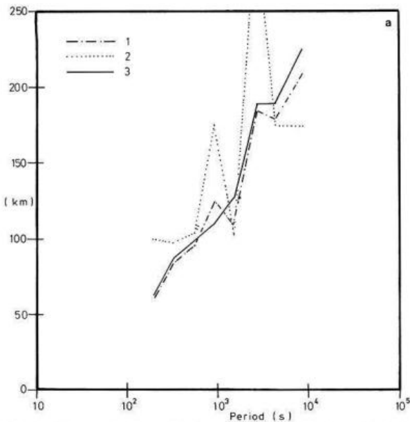
Fig. 4. a Determinations of g from the three methods outlined in Sect. 3; (---) method 1, (.....) method 2, (—) method 3. b As for (a) but for h
