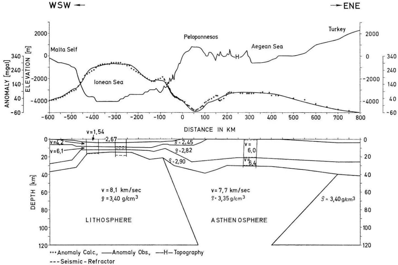
Fig. 1. 2-D crustal model between the Malta Shelf and Turkey. Seismic data in the Jonian Sea and Greece, see text. Gravity values give Bouguer anomalies
