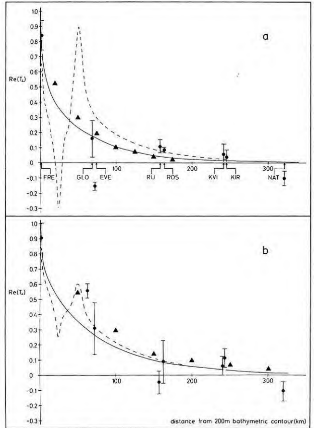
Fig. 13a, b. Dots indicate the magnitude of the real part of the inductive transfer function at a 200 s and b 1,000 s in the direction parallel to AA', i.e., perpendicular to the coast, or E -polarisation, for the stations FRE, GLO, EVE, RIJ, ROS, KVI, KIR, and NAT, as compared to the distance from the 200 m bathymetric contour west of FRE (see Fig. 12). The ranges are the 68 % confidence intervals of the rotated functions. Triangles indicate the Fischer first-approximation of a perfectly conducting thin sheet overlying a half space at a 200 s and b 1,000 s for half-spaces of 230 \Omega\text{m} and 130 \Omega\text{m} respectively. Full lines are the Schmucker thin-sheet modelling results for the model shown in Fig. 14 without a Vestfjord representation. Dashed lines are the Schmucker thin-sheet modelling results for the model shown in Fig. 14 with a tau representation of Vestfjord (see text)
